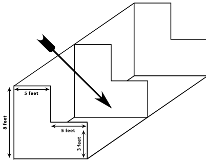
Correct Set-up
